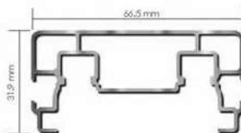
Dimensions rail M40
